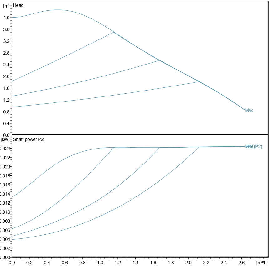
Performance according to ISO 9906:2012 – Grade 3B Liquid temperature: Power data referred to: Water [100%]; 4°C; 1000kg/m 3 ; 1.57mm 2 /s
