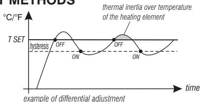
example of differential adjustment
